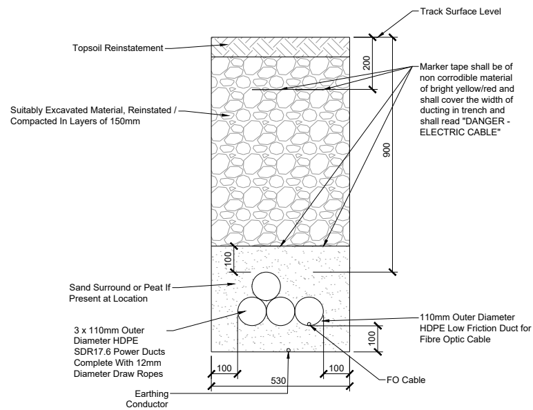
COLLECTOR CIRCUIT VERGE
