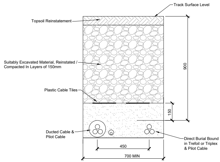
TRENCH CROSS SECTION - PILOT CABLES
