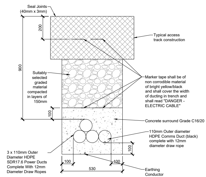
COLLECTOR CIRCUIT CENTRE
