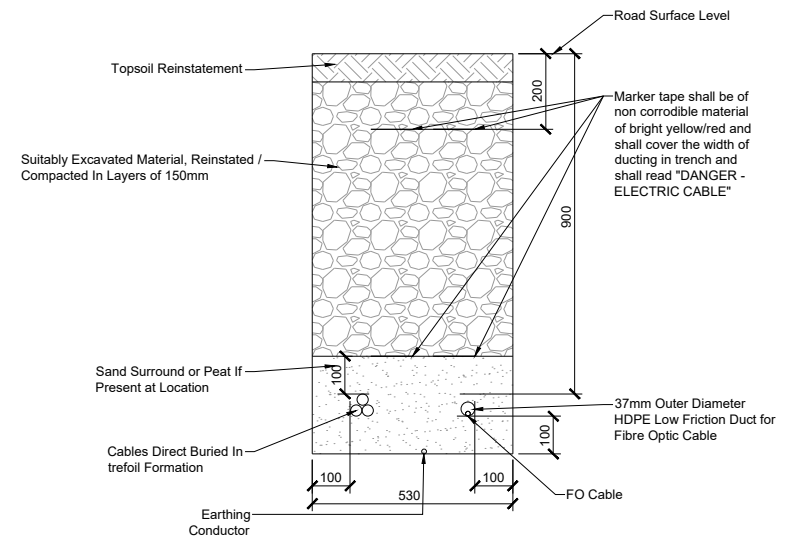
COLLECTOR CIRCUIT VERGE (DIRECT BURY)
